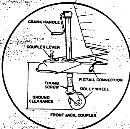
FRONT JACK FIGURE 1
