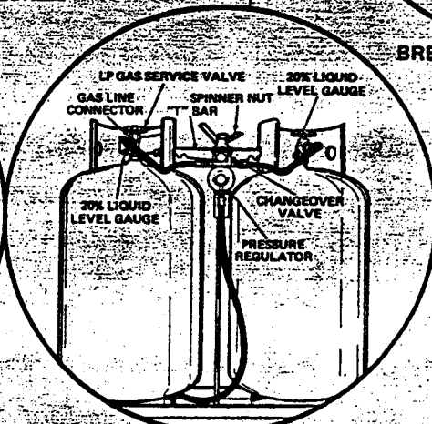
DUAL LP GAS BOTTLES FIGURE 16
