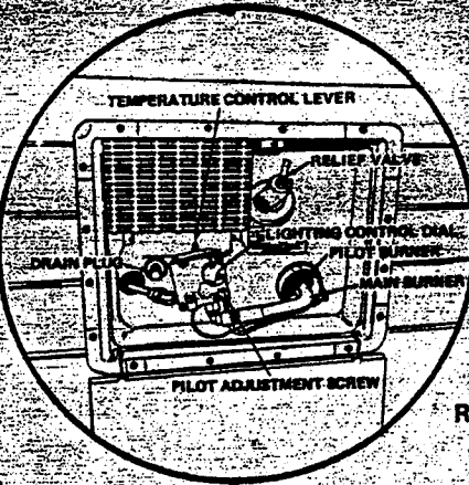
WATER HEATER (HYD) FIGURE 19
