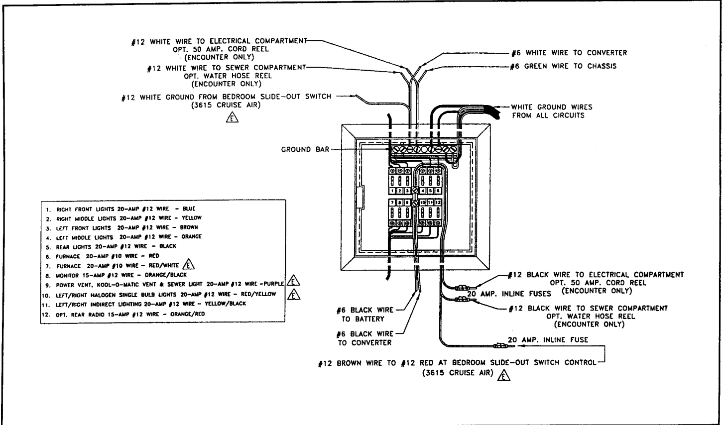
Typical 12-Volt 12-Circuit Power Converter Fuse Panel (CSA)
