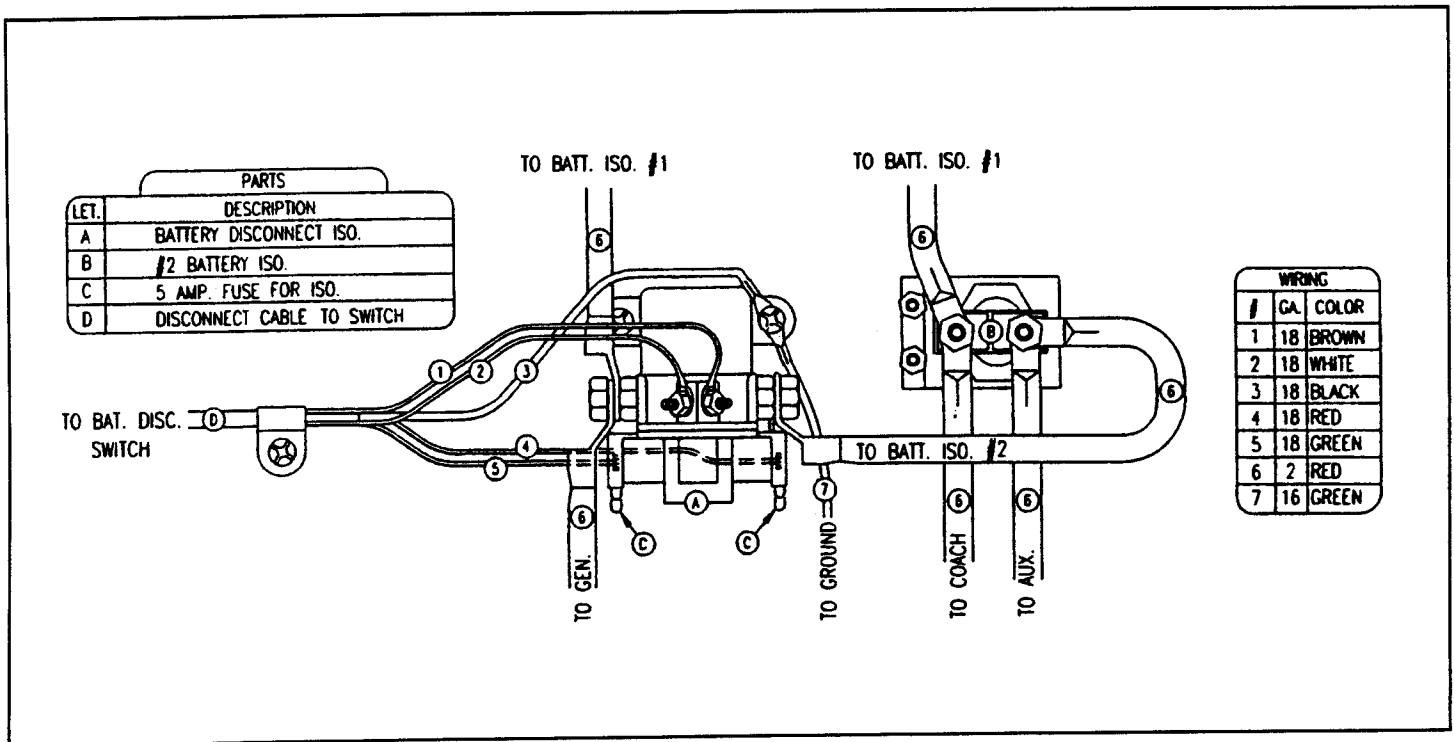
Typical Auxiliary Battery Disconnect Circuit
