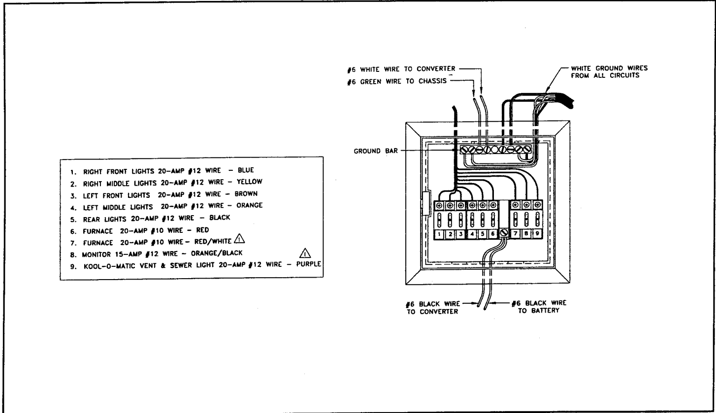
Typical 12-Volt 9-Circuit Power Converter Fuse Panel
