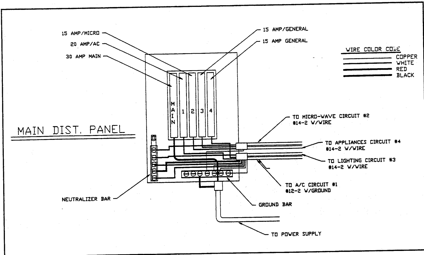
Typical 115-Volt 30-Amp Electrical Circuit
