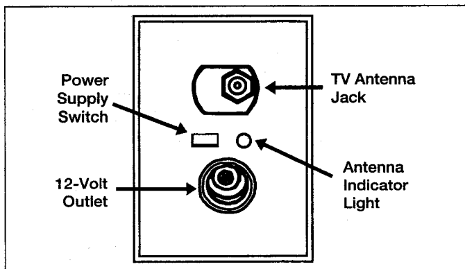
TV WALL PLATE
