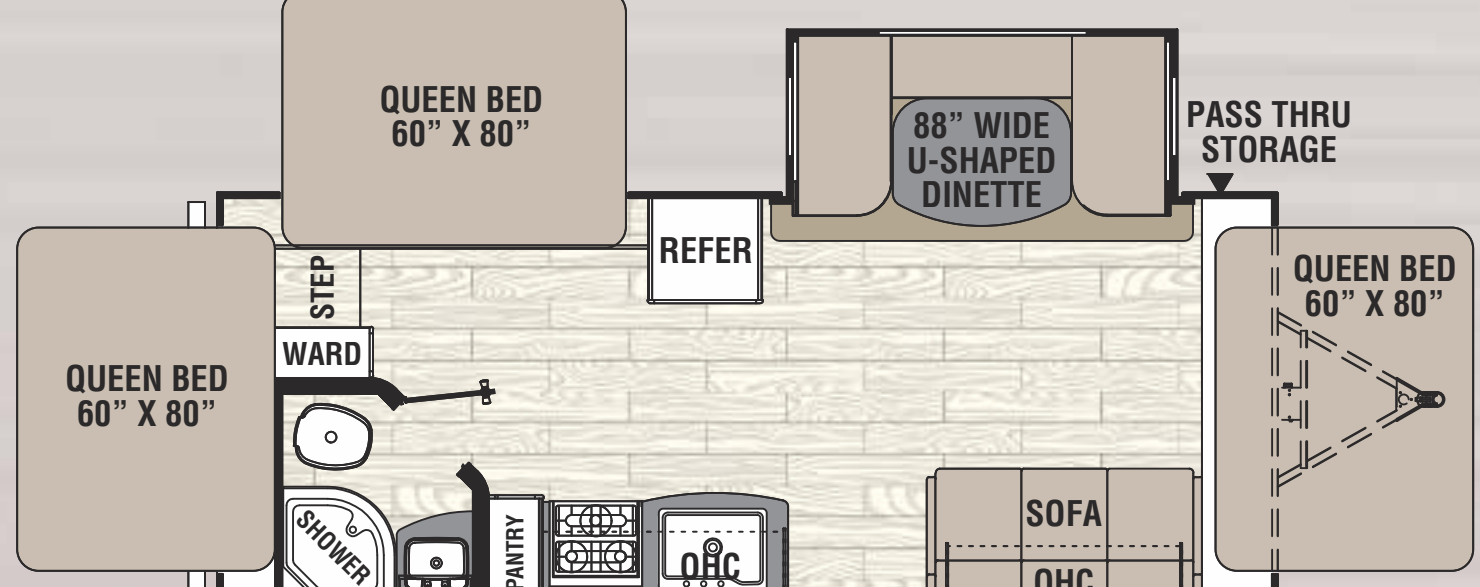
23 TQX / Exterior Length 24' 3"
