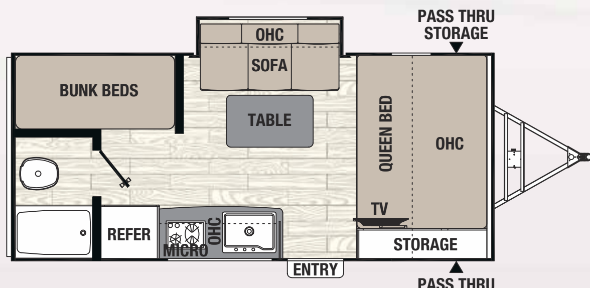
20 BHS / Exterior Length 22'
