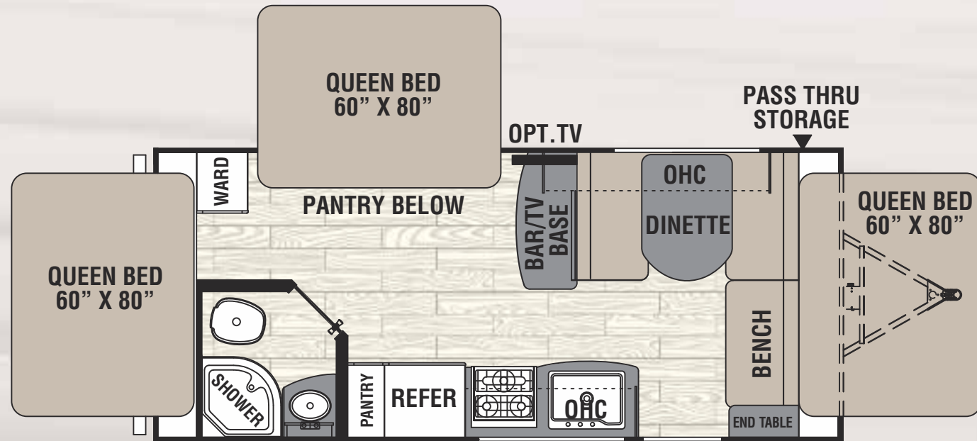
21 TQX / Exterior Length 22' 7"
