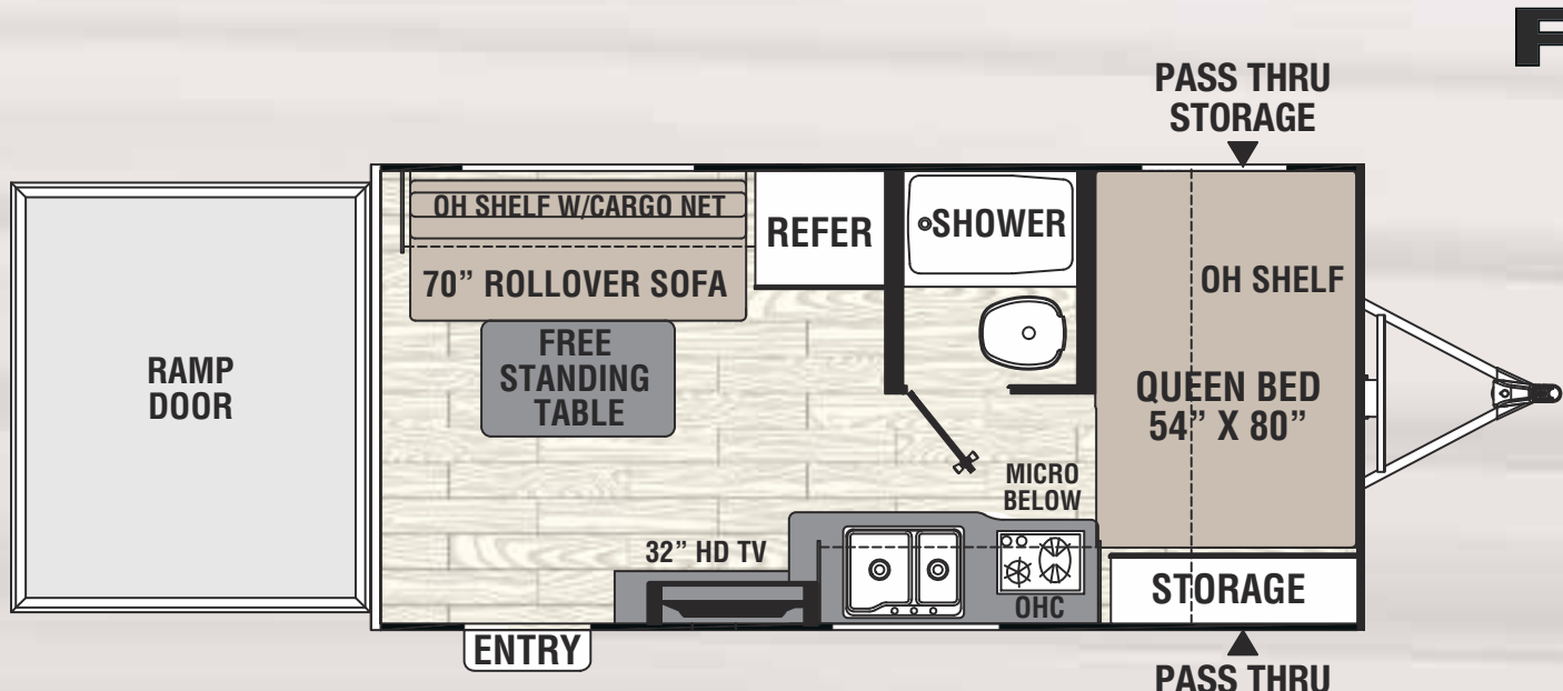
17 BLSE / Exterior Length 20' 4"
