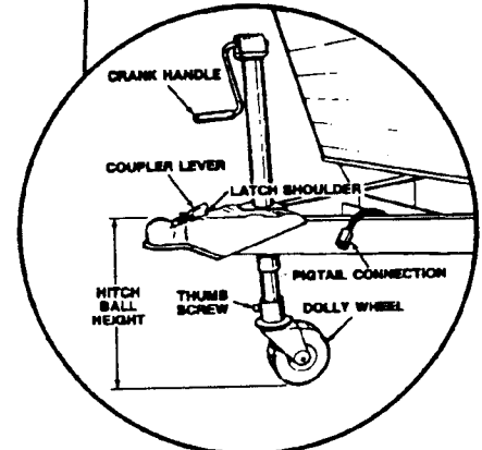
FRONT JACK FIGURE 8
