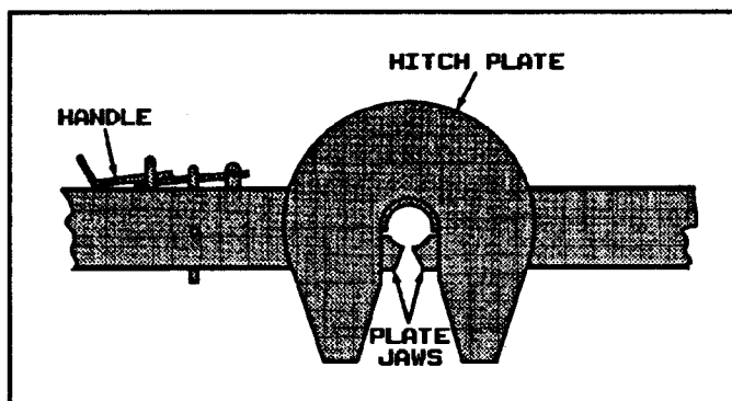
FIFTH WHEEL PLATE (TYPICAL)
