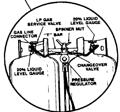
DUAL LP GAS BOTTLES FIGURE 21
