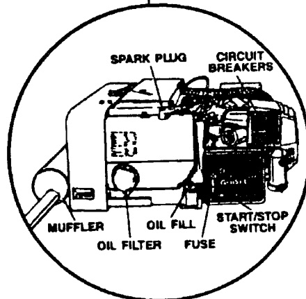
GENERATOR FIGURE 22
