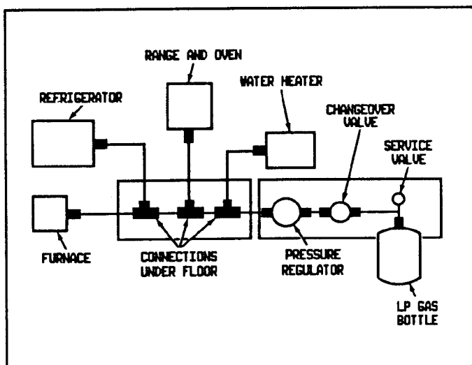
LP GAS SYSTEM (TYPICAL)
