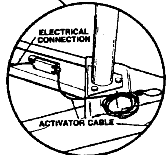
BREAKAWAY SWITCH FIGURE 5
