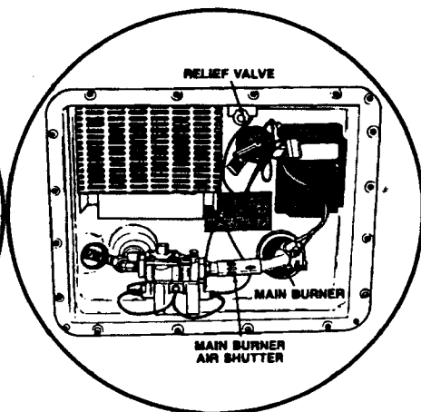
WATER HEATER (ELECTRONIC IGNITION) FIGURE 17
