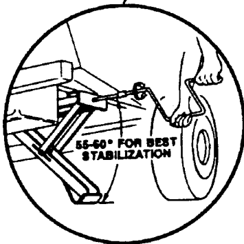
STABILIZING JACKS FIGURE 9
