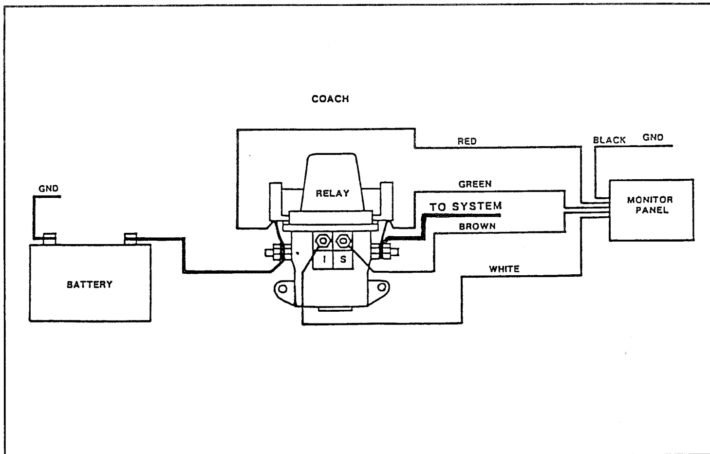
Typical Auxiliary Battery Disconnect Circuit
