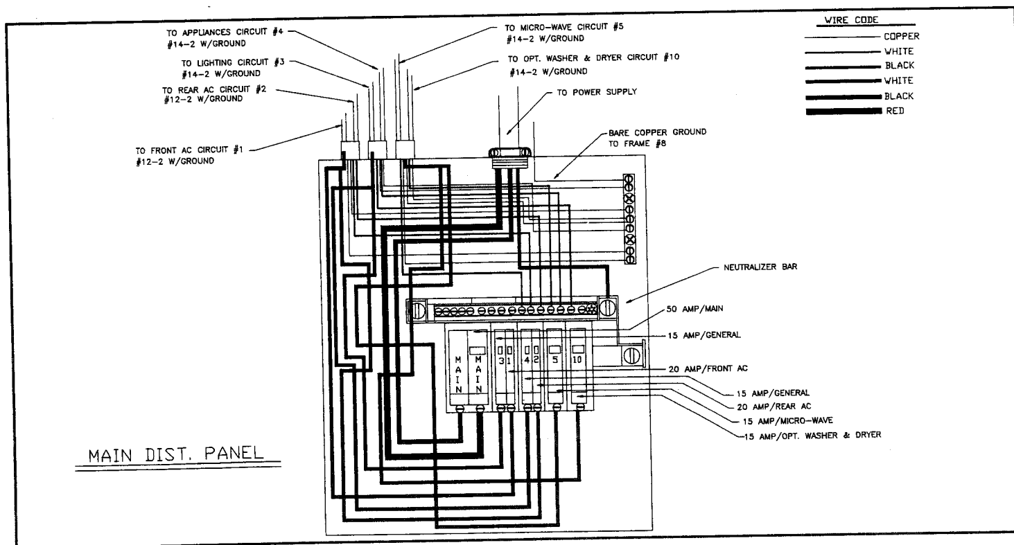
Typical 115-Volt 50-Amp Electrical Circuit
