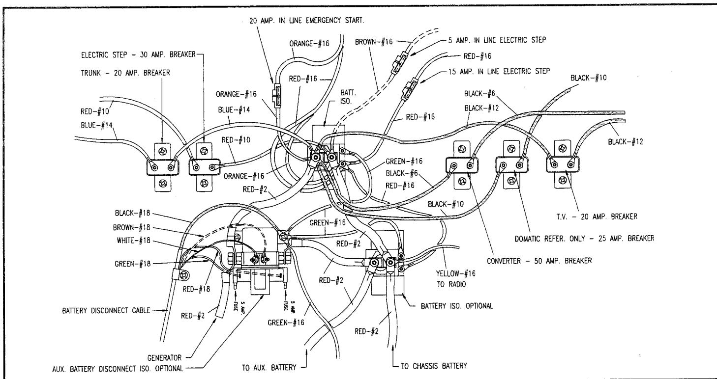
Typical Automotive Electric Circuit
