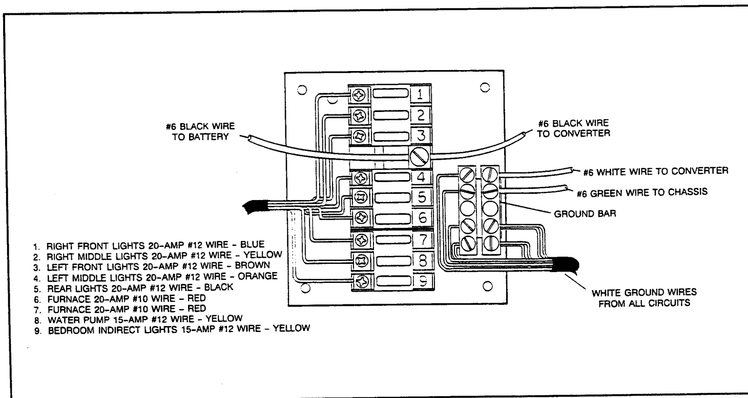
Typical 12-Volt 9-Circuit Power Converter Fuse Panel
