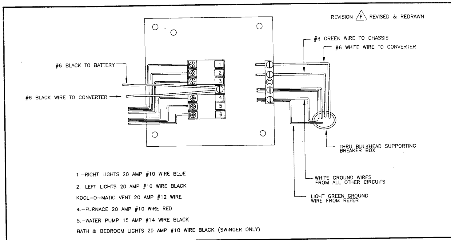
Typical 12-Volt 6-Circuit Power Converter Fuse Panel
