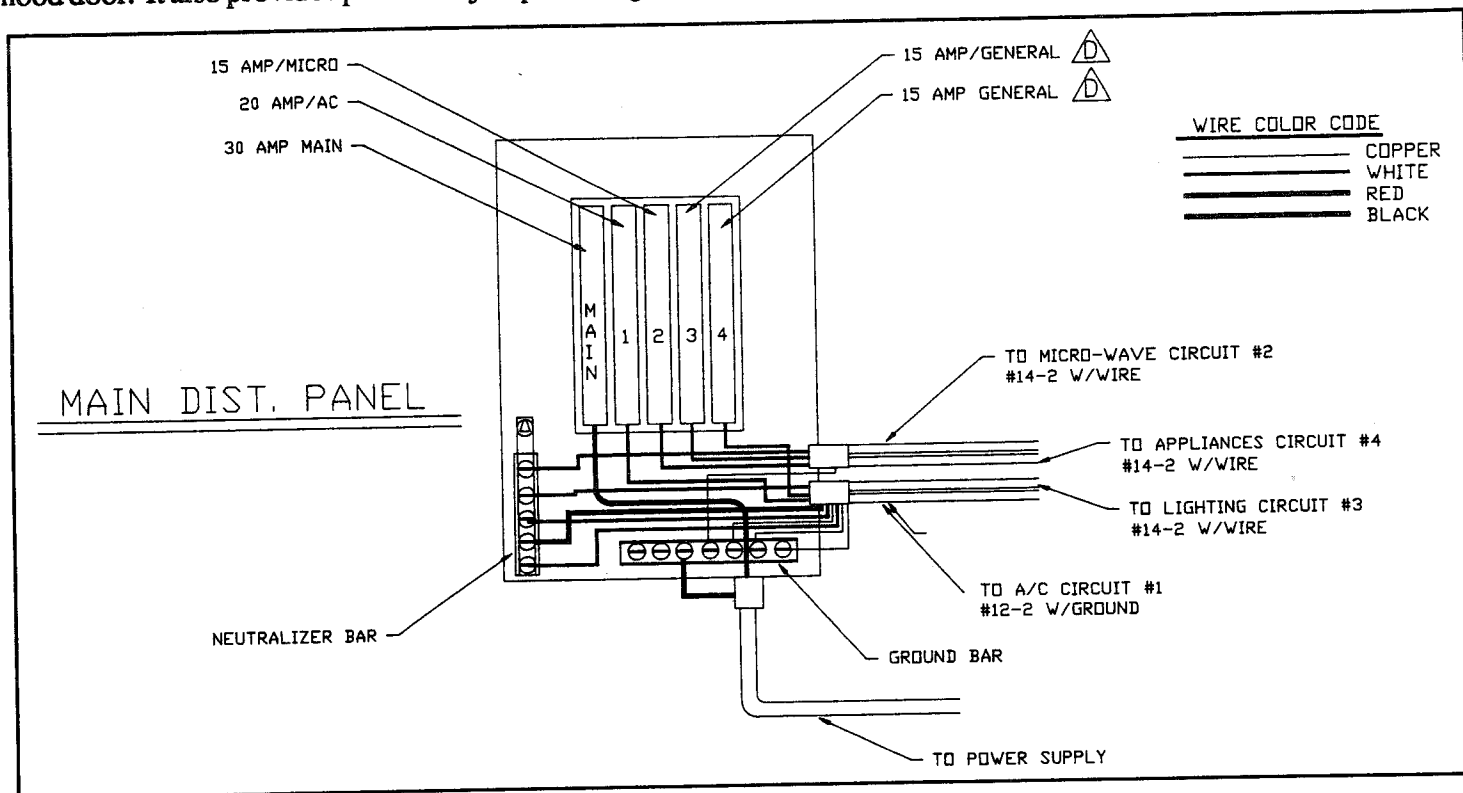
Typical 115-Volt 30-Amp Electrical Circuit
