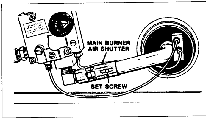
WATER HEATER BURNER ADJUSTMENT
